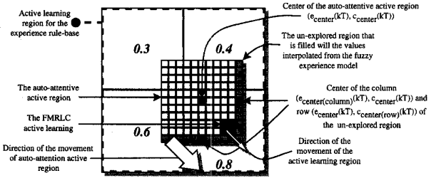
Fig. 26. DFL III: The enlargement of the active learning region for the experience rule-base.
