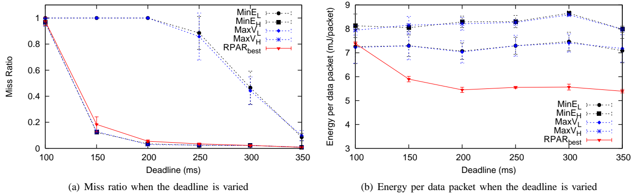
Fig. 2. Performance of considered protocols when deadline is varied. The neighborhood table is prefilled.
