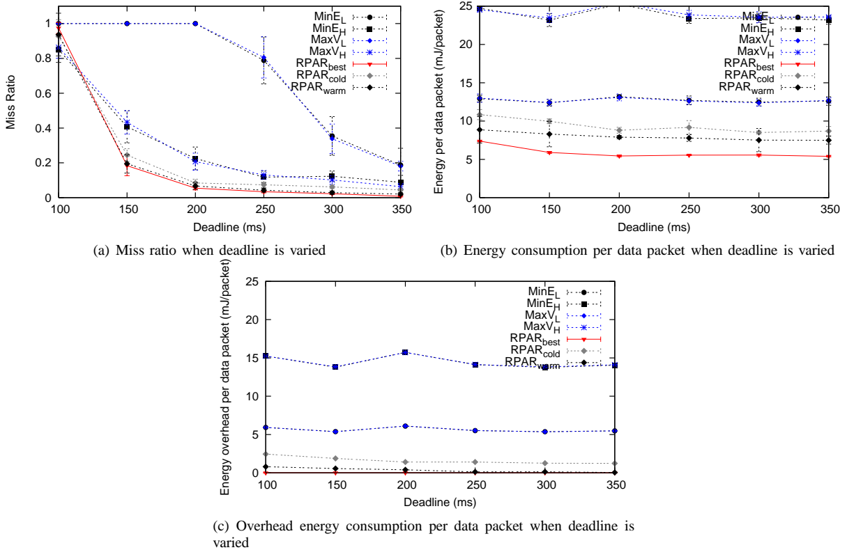
Fig. 3. Performance of considered protocols when deadline is varied (with neighborhood management).
