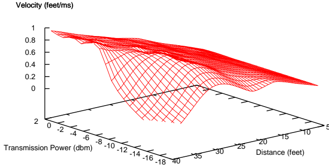
Fig. 1. Impact of transmission power and one-hop distance on delivery velocity.
