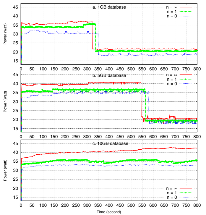
Fig. 5. Power consumption of the TPC-C workloads under three different database sizes.
