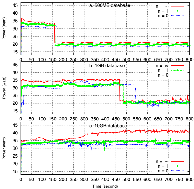
Fig. 4. Power consumption of the TPC-H workloads under three different database sizes.
