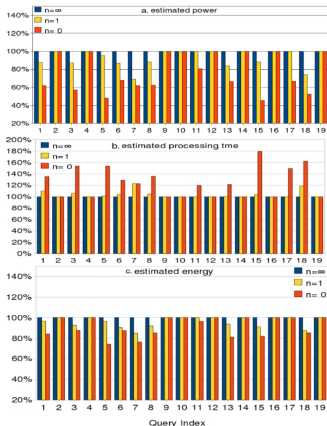
Fig. 6. Power and processing time of the chosen plans for the 19 queries in the TPC-H benchmark as estimated by the query optimizer. Data presented as relative values to the n = \infty case. Note here some figures shown here and later start their y axes at 2 / 20% for emphasize the difference.
