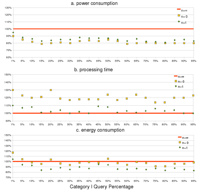
Fig. 8. Relative quantity of power, processing time and energy consumption under workloads with different category I to II query ratios.
