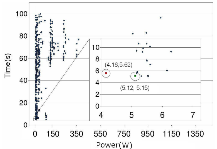
Fig. 2. The estimated processing time and power cost of plans evaluated by the modified PostgreSQL query optimizer for the query shown in Fig. 1. The small graph is a magnification of the bottom left portion of the large graph. Even the big graph contains only 1/5 of the plans visited by the query optimizer. The other 4/5 is ignored due to their inferiority (in both performance and energy).
