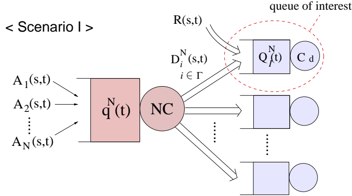
Figure 1. Queueing network: Scenario I
