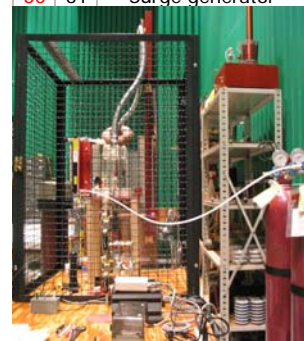
Surge generator
