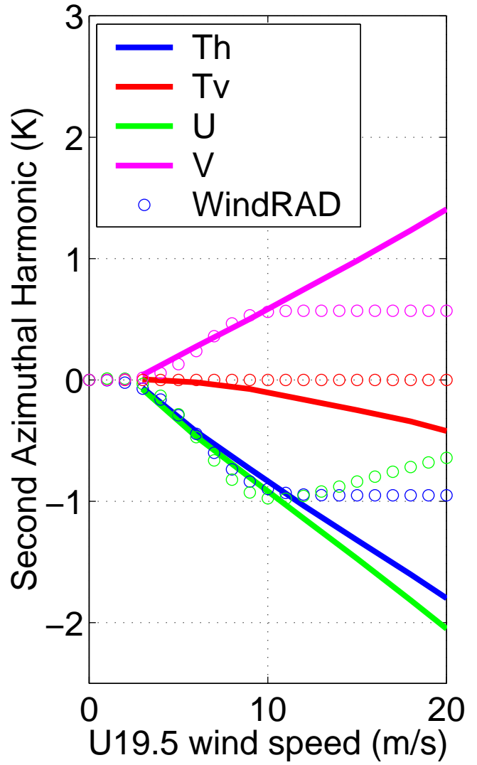
19.35 GHz, 55°
