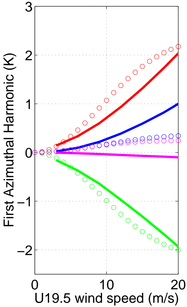
19.35 GHz, 55°
