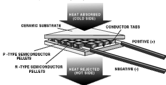
Multi-couple configuration increases heat-pumping capacity
