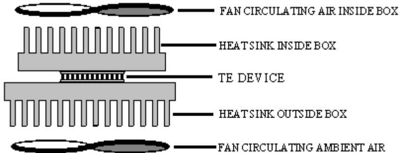
Conceptual Drawing of Air-to-Air Thermoelectric Cooling System
