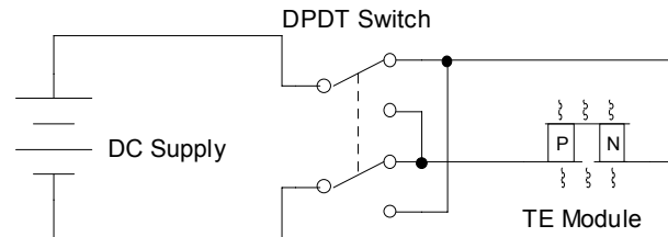
Polarity Reversal Configuration
