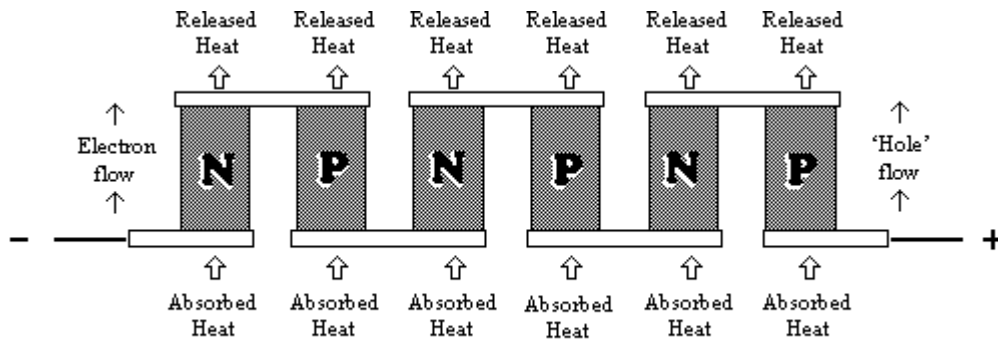
Multi-couple configuration increases heat-pumping capacity
