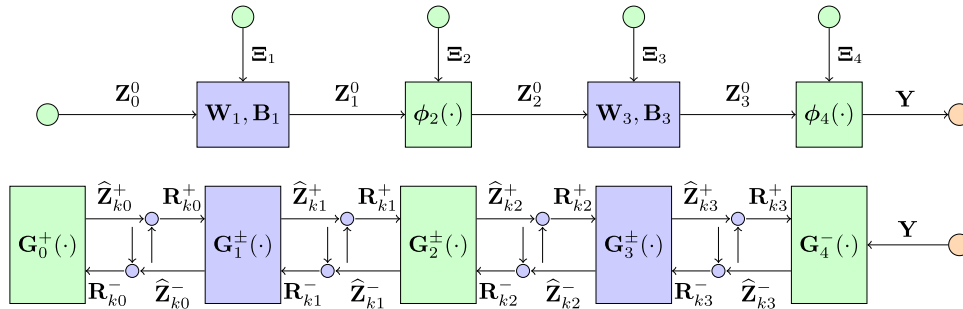
Figure 1. (Top) The signal flow graph for true values of matrix variables \{\mathbf{Z}_\ell^0\}_{\ell=0}^3 , given in equation (1) where \mathbf{Z}_\ell^0 \in \mathbb{R}^{n_\ell \times d} . (Bottom) Signal flow graph of the ML-MVAMP procedure in algorithm 1. The variables with superscript + and – are updated in the forward and backward pass respectively. ML-MVAMP (algorithm 1) solves (2) by solving a sequence of simpler estimation problems over consecutive pairs (\mathbf{Z}_\ell, \mathbf{Z}_{\ell-1}) .
