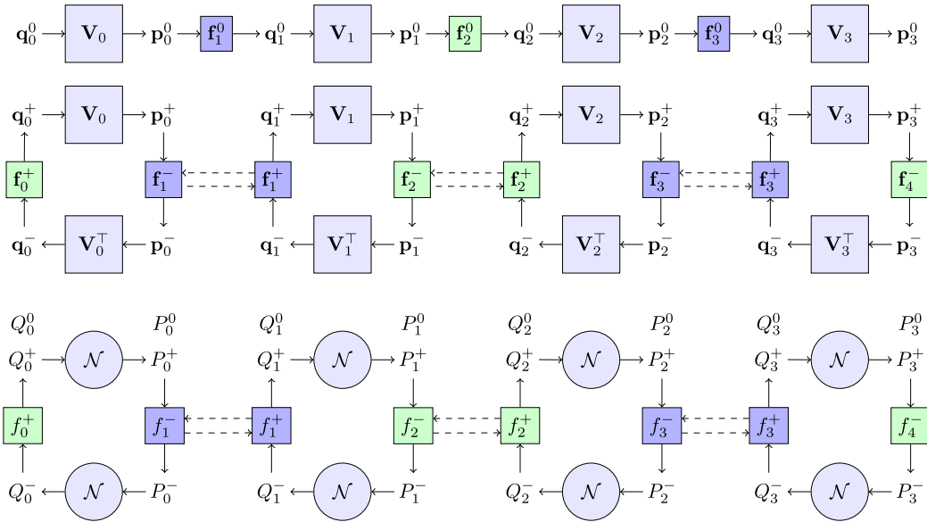
Figure 3. (Top) The equation (1) with equivalent quantities defined in (23), and f_l^0 defined using (19). (Middle) The Gen-ML-Mat recursions in algorithm 3. These are also equivalent to ML-Mat-VAMP recursions from algorithm 1 (see lemma 1) if q_l^\pm, p_l^\pm are as defined as in equations (24) and (26), and f_l^\pm given by equations (20) and (21). (Bottom) Quantities in the GEN-ML-SE recursions. These are also equivalent to ML-Mat-VAMP SE recursions from algorithm 2 (see lemma 1). The iteration indices k have been dropped for notational simplicity.
