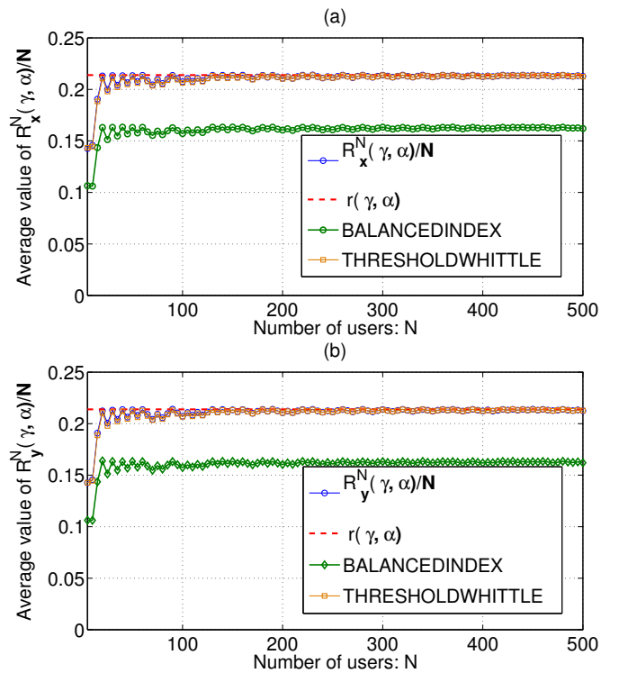
Fig. 6: Performance evaluation and comparison of per-user throughput of Whittle's Index Policy. (a) Z^N[0] = \mathbf{x} ; (b) Z^N[0] = \mathbf{y} .
