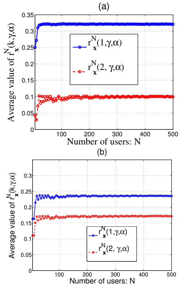
Fig. 7: Evaluation of r_x^N(k, \gamma, \alpha) with N . (a) Whittle's Index Policy; (b) Policy \Xi .
