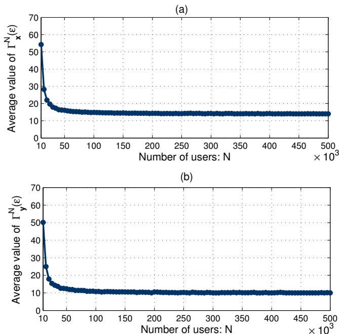
Fig. 4: Average time of hitting \Omega_\epsilon(\vec{\zeta}_\gamma^\alpha) . (a) \mathbf{Z}^N[0] = \mathbf{x} ; (b) \mathbf{Z}^N[0] = \mathbf{y} .
