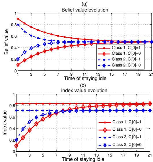
Fig. 5: The evolution of belief value and Whittle's index value. (a) Belief value evolution (b) Whittle's index value evolution.
