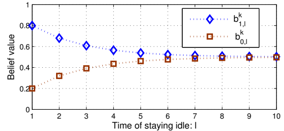
Fig. 2: Belief values update when staying idle, p_k = 0.8 , r_k = 0.2 , b_s^k = 0.5 .
